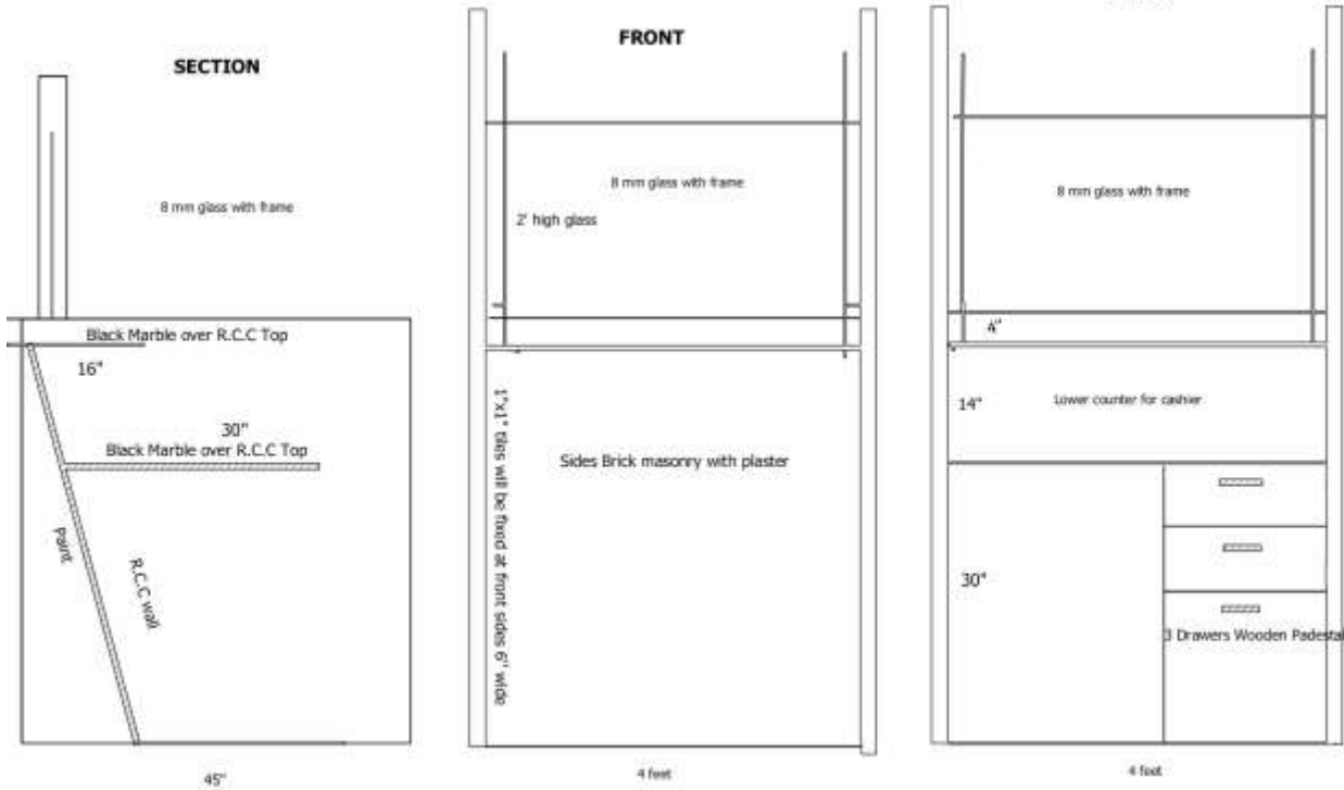
BRICK/R.C.C CASH COUNTER DETAILS
